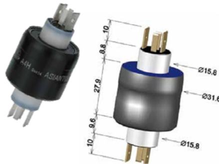
A4H 2poles/30A & 2poles/4A AC250V
