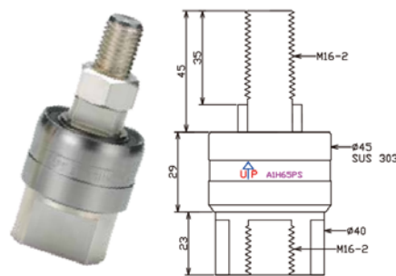
A1H65PS 1pole 650A
